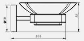
Zinc alloy + glass cup, chrome plated
