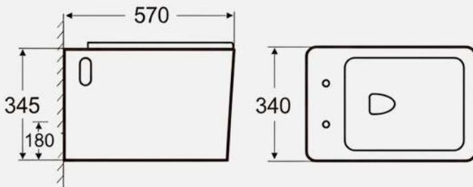
8541W Wall Hung Toilet Size: 570*340*345 MM P-trap: 180mm Roughing in
